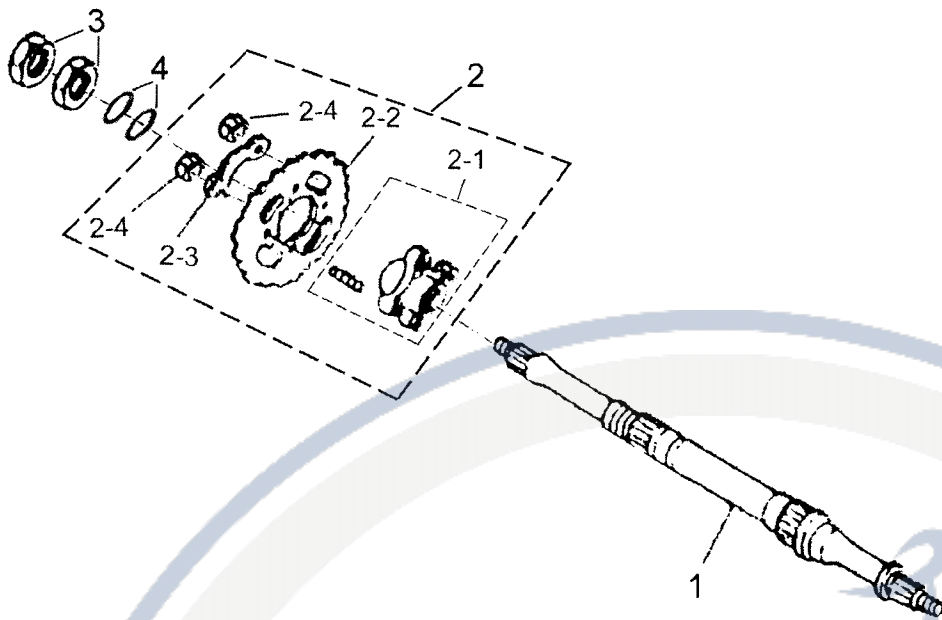
Drawing No: 028-008
